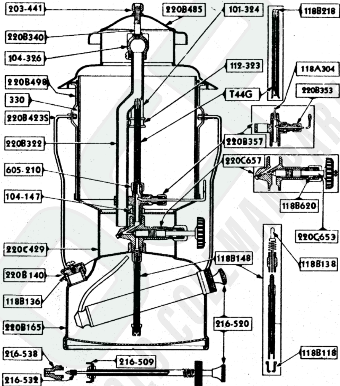
INSTANT-LITE LANTERN Model No. 220C
